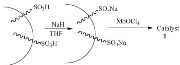
Scheme 1 Immobilization of MoOCl 4 to the Nafion support.
